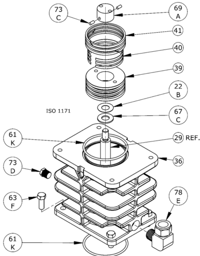
Cylinder Assembly: Model LB081B, LB082B
