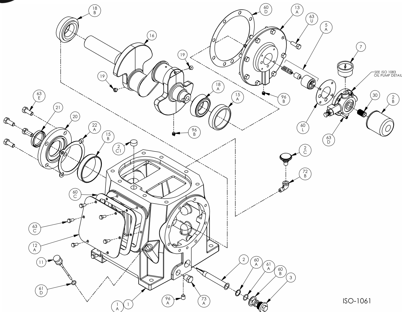
Crankcase Assembly: Models HD942A, HD942B, HDL942A, HDL942B
