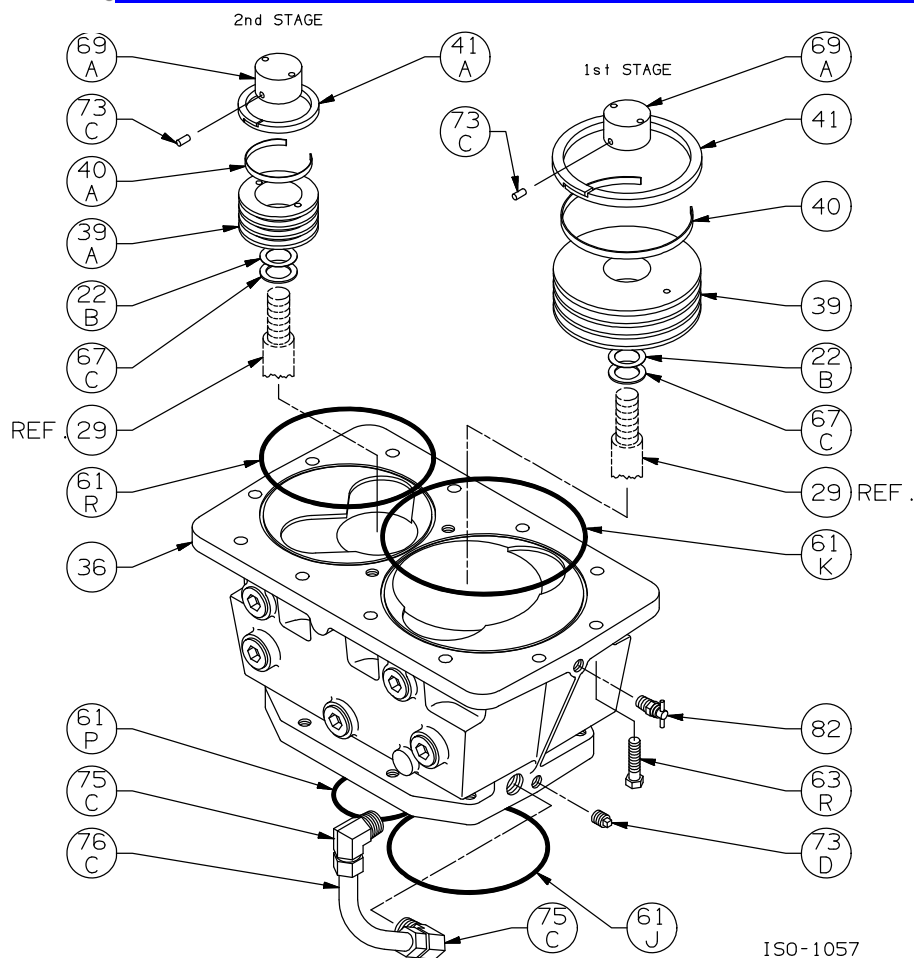
Cylinder Assembly: HDL612C|B|A, HDL613C|B
