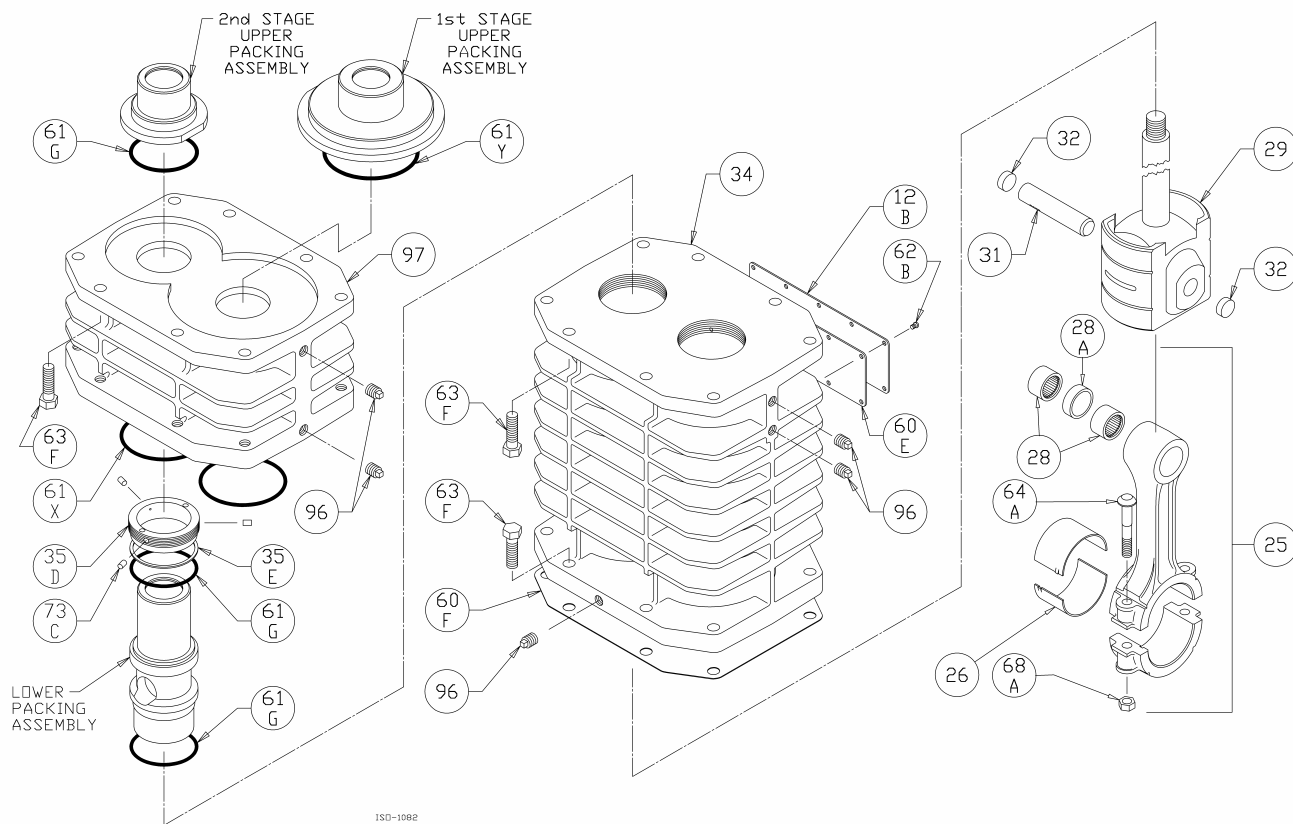
Crosshead Assembly: HD613C, HDL613C
