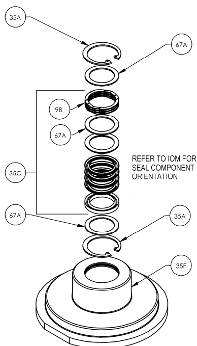
UPPER PACKING ASSEMBLY 1st STAGE
