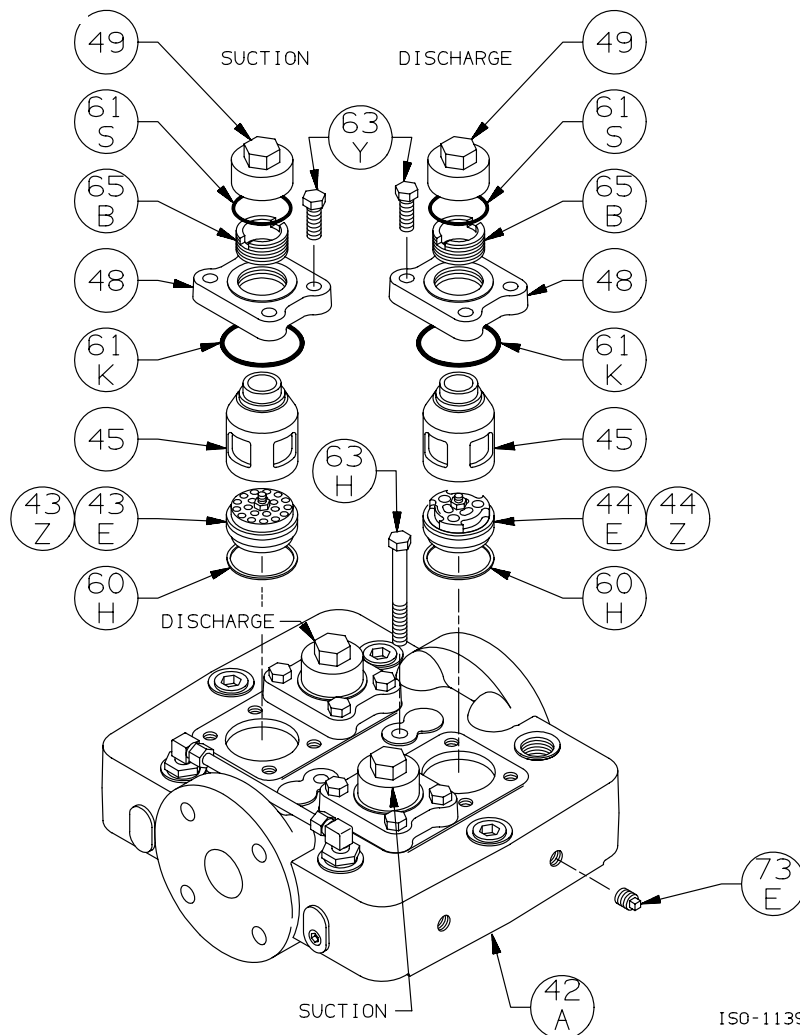
Head Assembly: Models HDL362C, HDL363C
