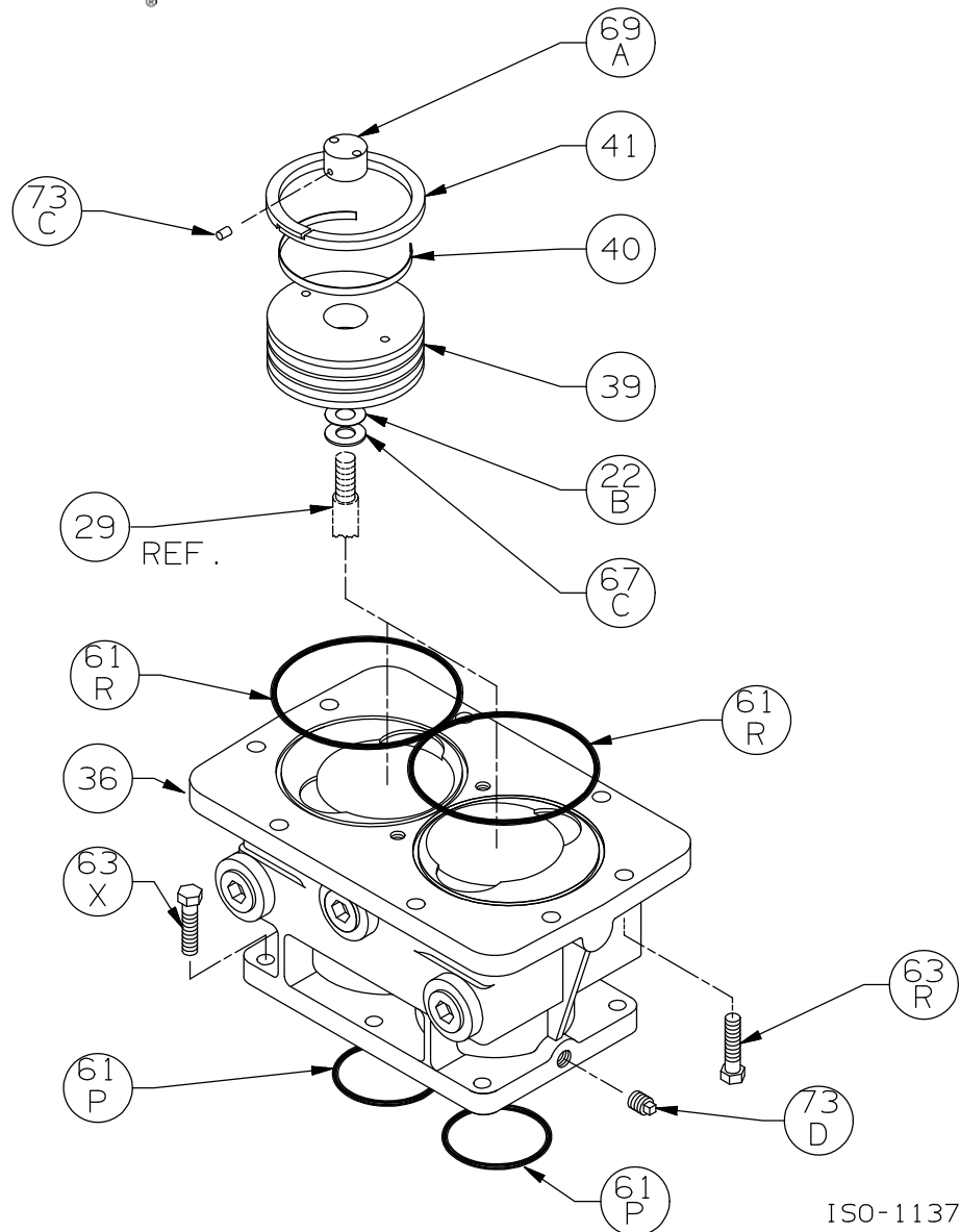
Cylinder Assembly: Models HDL362C, HDL363C
