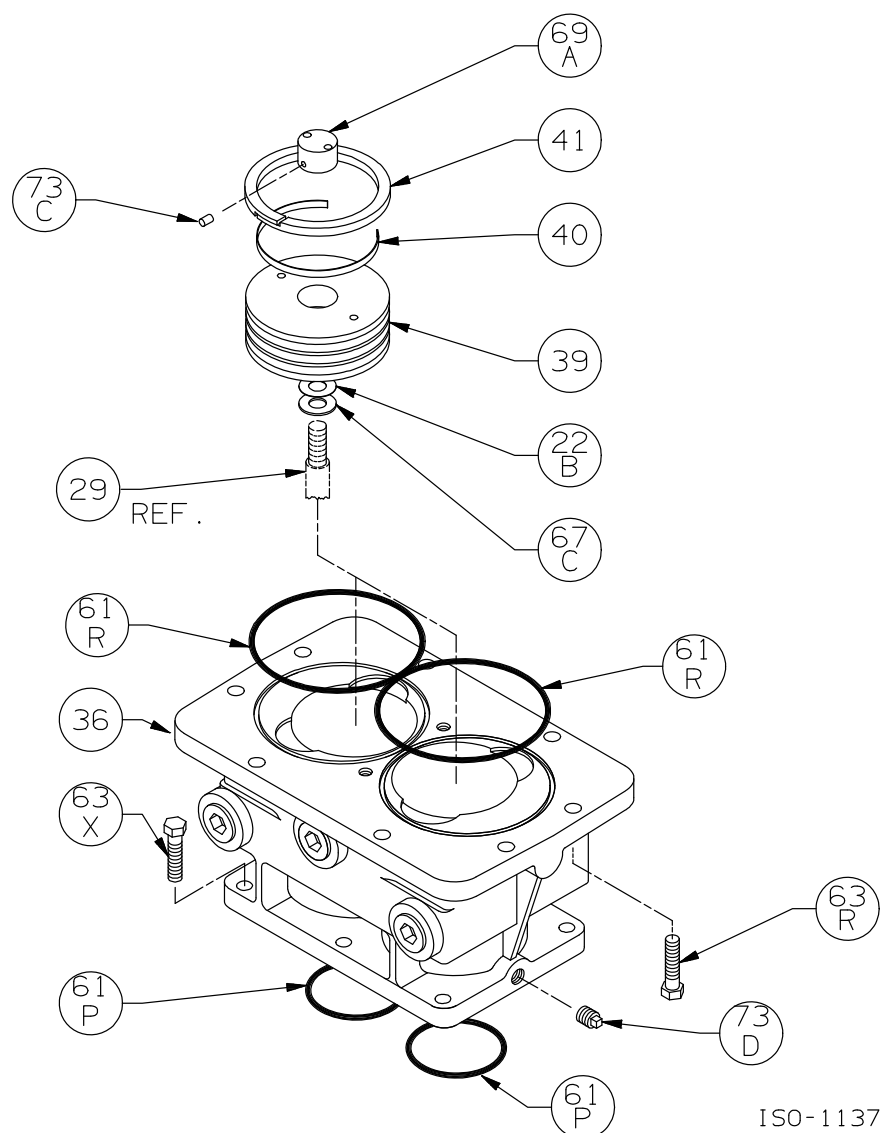
Cylinder Assembly: Models HDL322C, HDL323C
