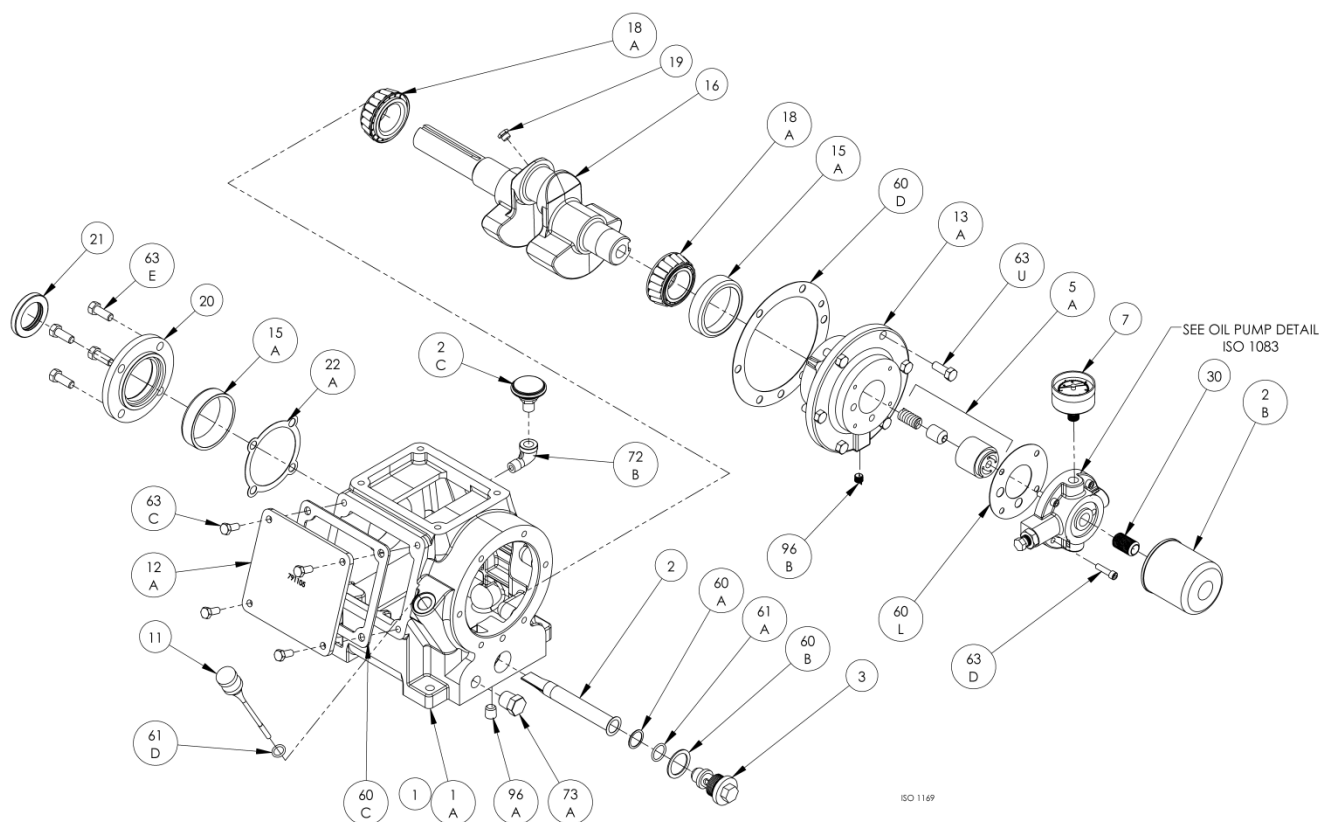
Crankcase Assembly: Models HD082C
