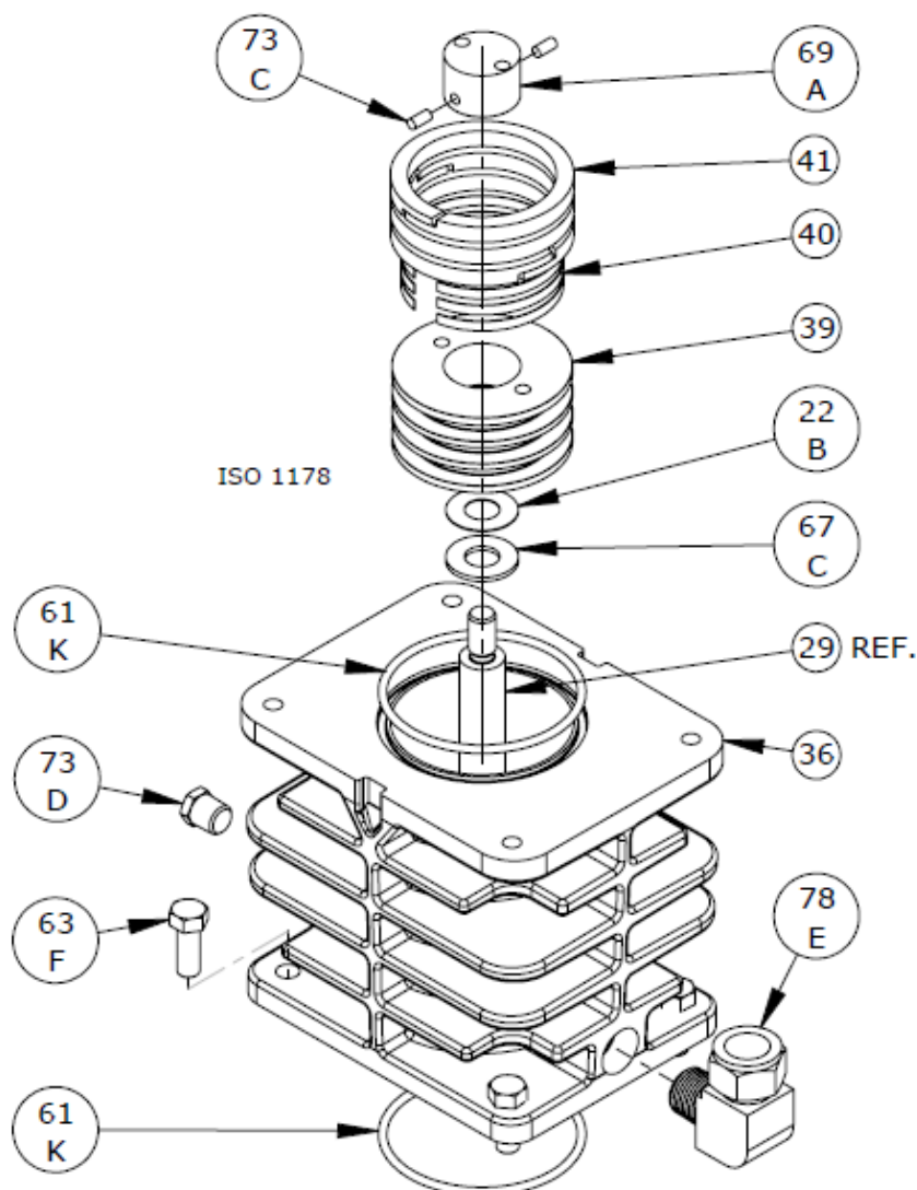
Cylinder Assembly: Model HD082C
