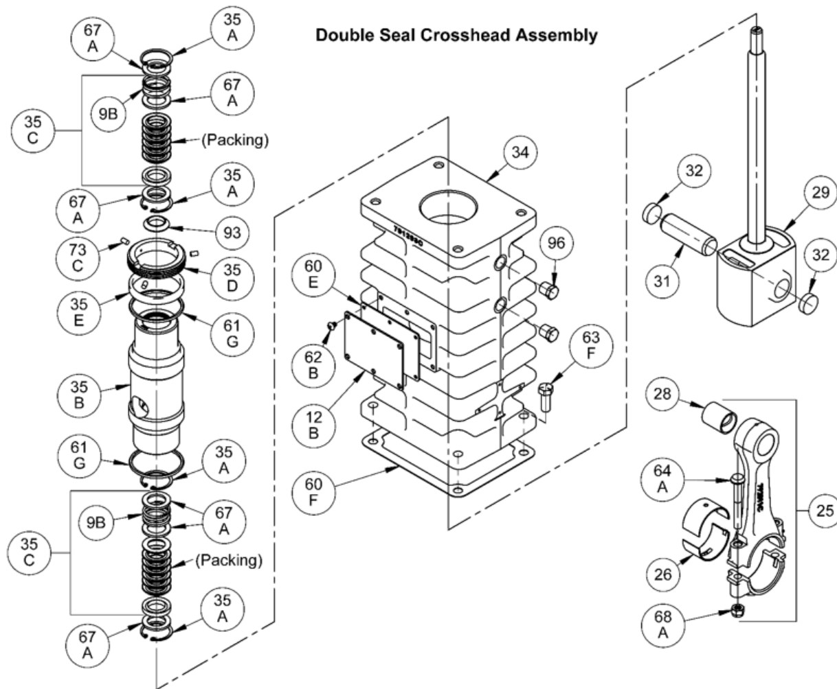
Crosshead Assembly: HD082C
