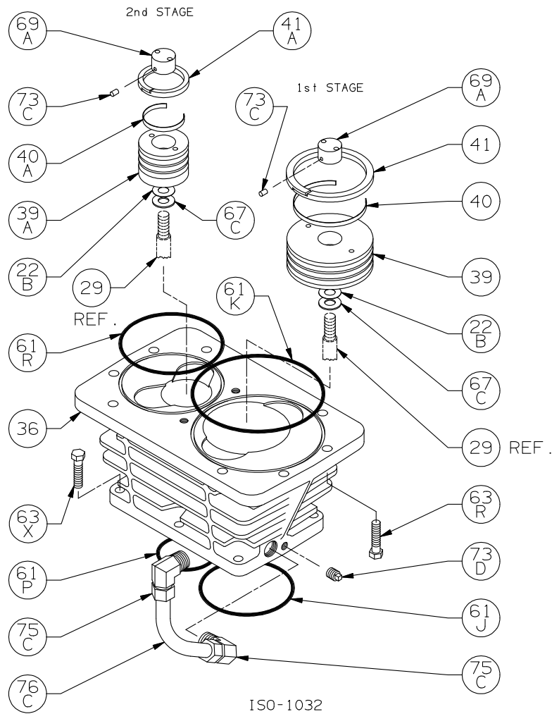
Cylinder Assembly: Model HDS372C
