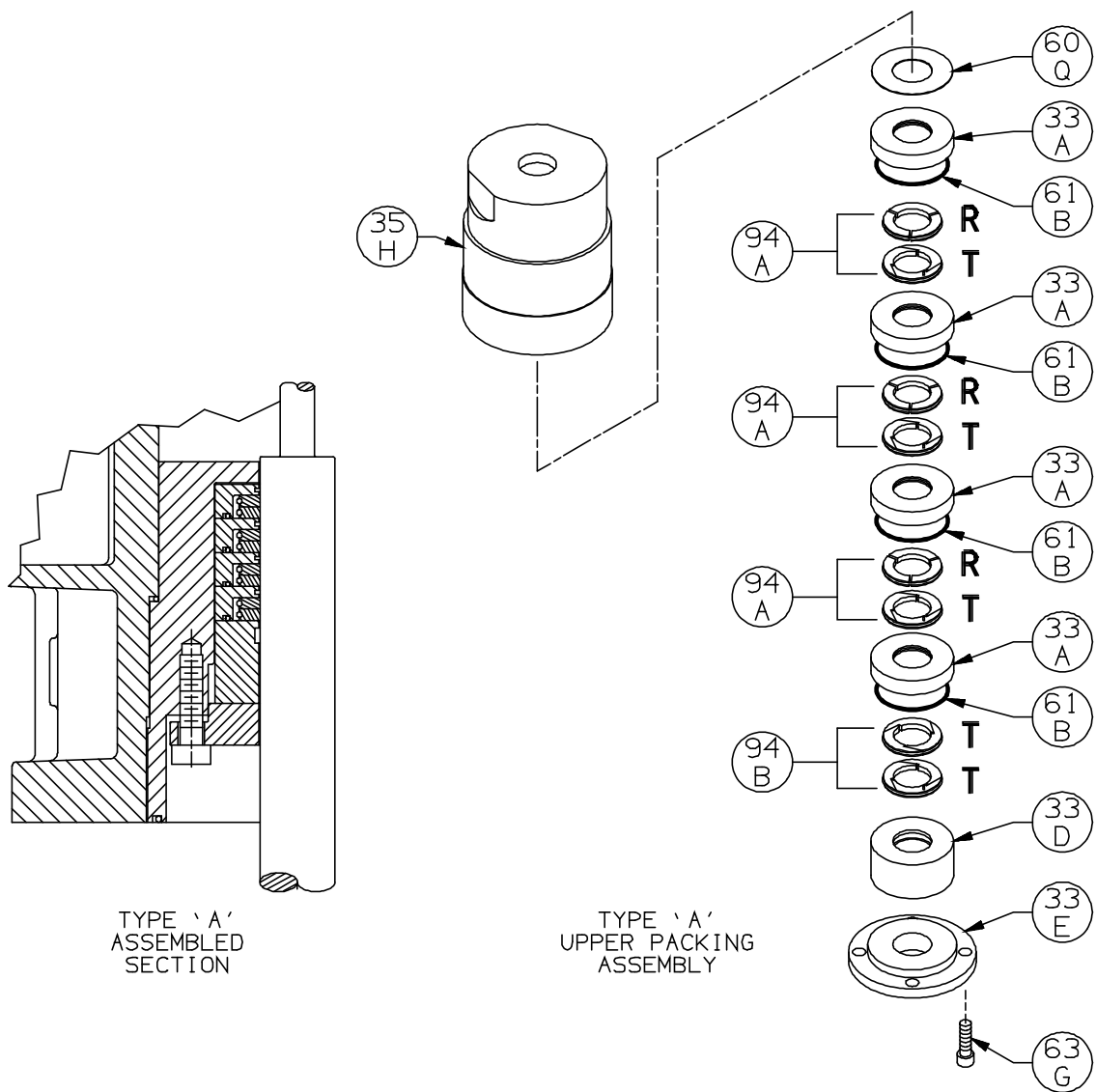
Upper Packing, Type 'A'
