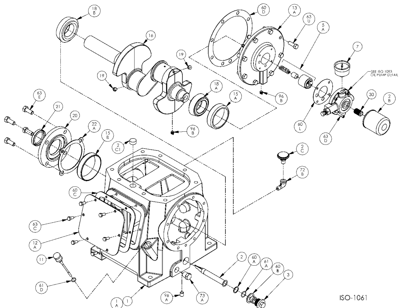
Crankcase ISO1061
