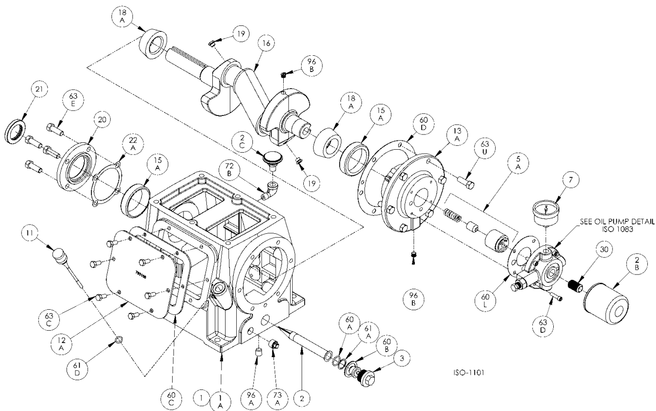
Crankcase ISO1101
