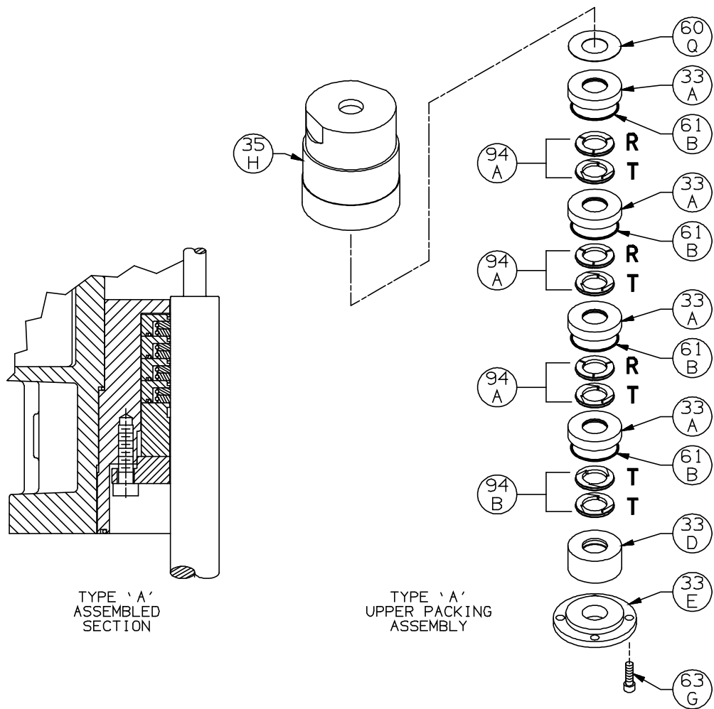
Upper Packing Box - Type 'A'
