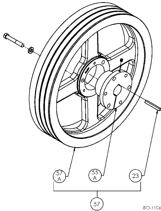
Flywheel S1106
