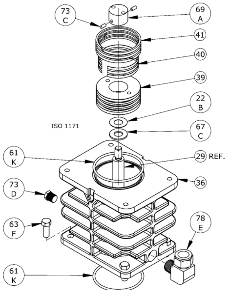
Cylinder Assembly: Model NG082B
