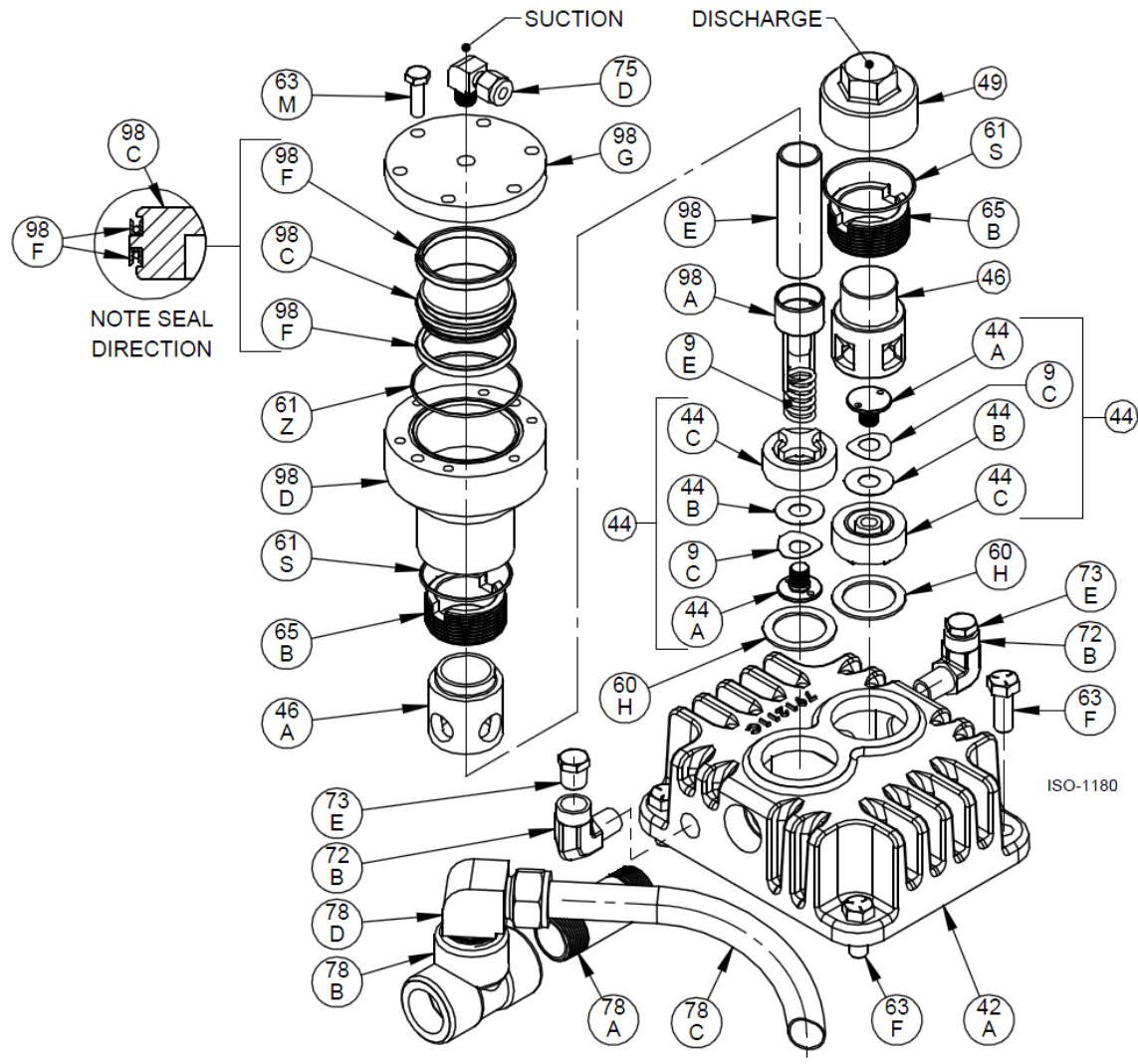
Head Assembly with Unloaders: Model NG082
