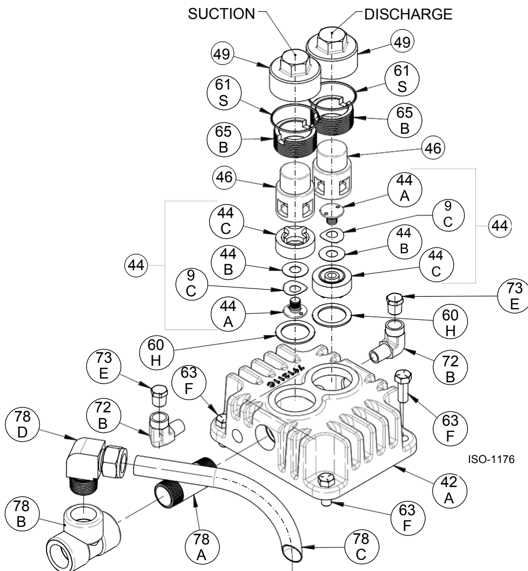
Head Assembly
