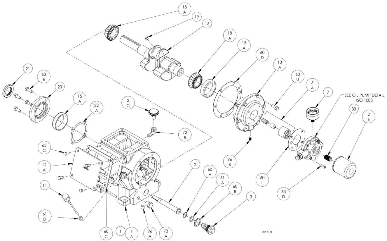
Crankcase Assembly: Models NG082B
