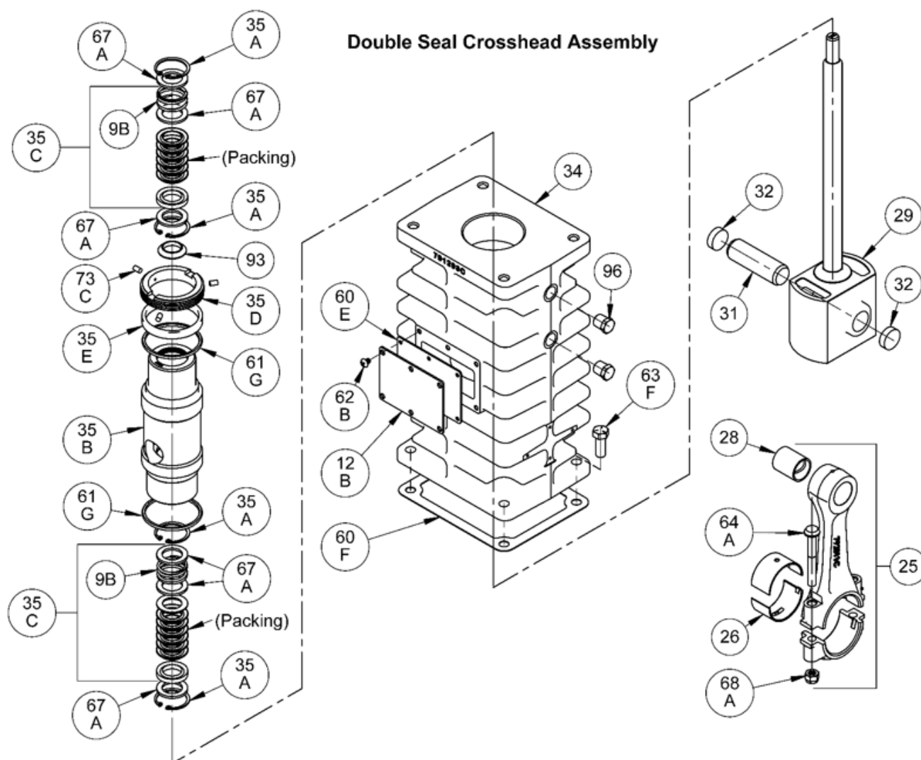
Crosshead Assembly: NG082B
